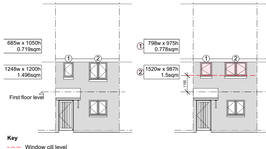
Figure 10. Case study house where cill heights were raised to 1100mm in order to meet the guarding standards of AD-O Table 3.1, and openings made wider (left: original design; right: raised cill heights). This changes external appearance and therefore would have planning implications: this is one example why Part O should be considered early in the design process; on sites with existing planning permission, the changes should be discussed with the Local Authority and in some cases may require a re-submission.
