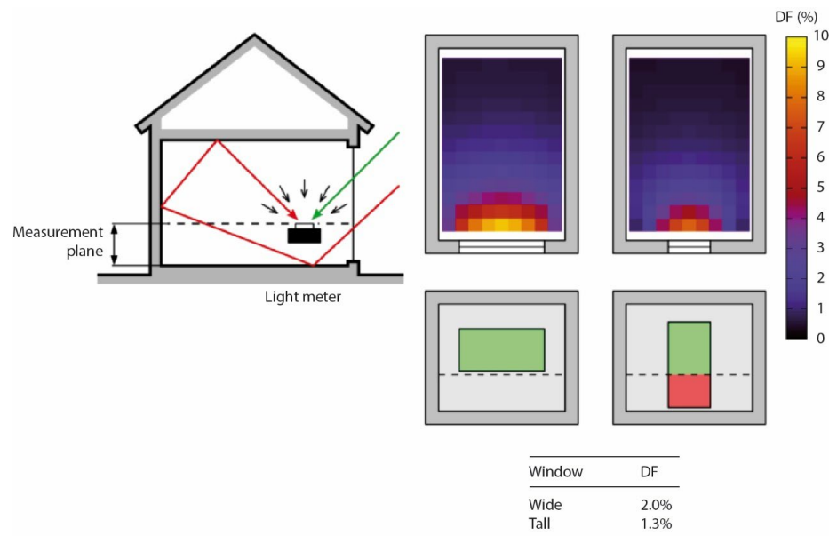
Figure 24. For daylight penetration and distribution into the room, glazing location matters, not just its amount (Illustration from Hoare Lea, CIBSE TM60, 2018).
