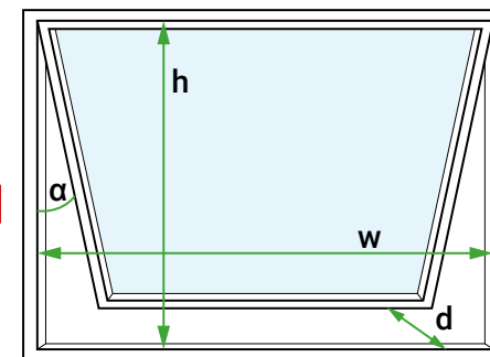
Figure 37. Illustration of using the Discharge coefficient calculator spreadsheet to determine equivalent area for the kitchen window.
