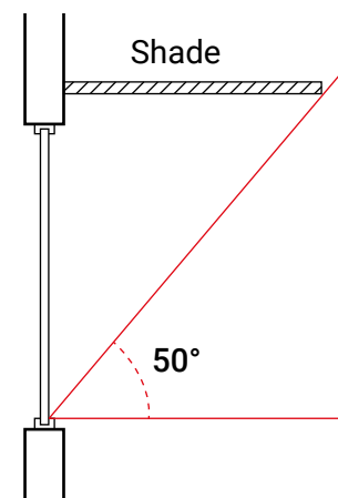
Figure 14. Illustration of "overhang with 50° altitude cut-off (from DLUHC FAQs, FAQ7).
