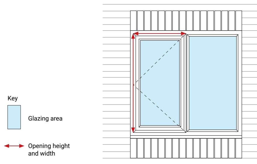
Figure 16. Illustration showing window measurements.
