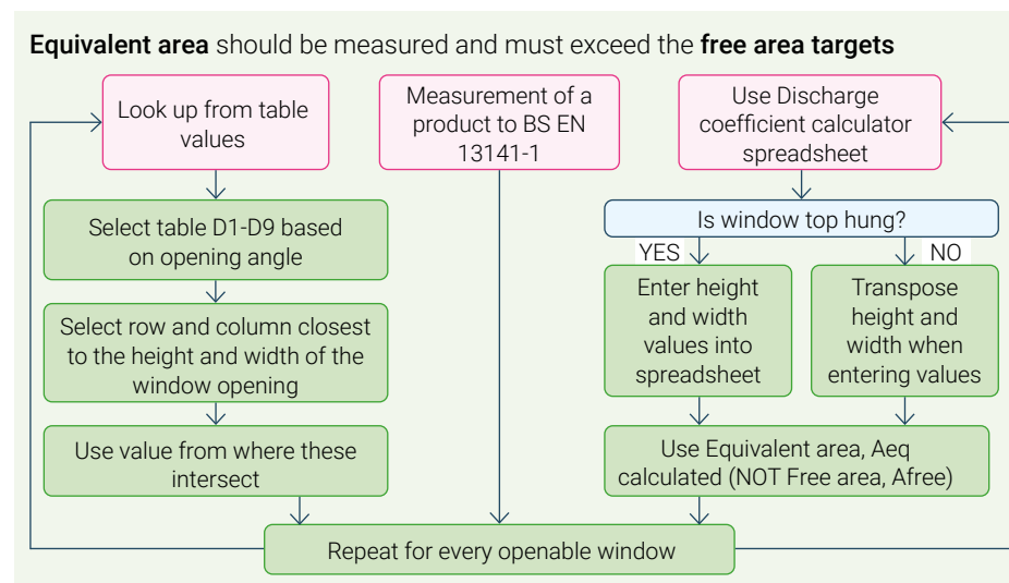
Figure 17. Illustration of the 3 possible methods to measure equivalent areas for Part O.
