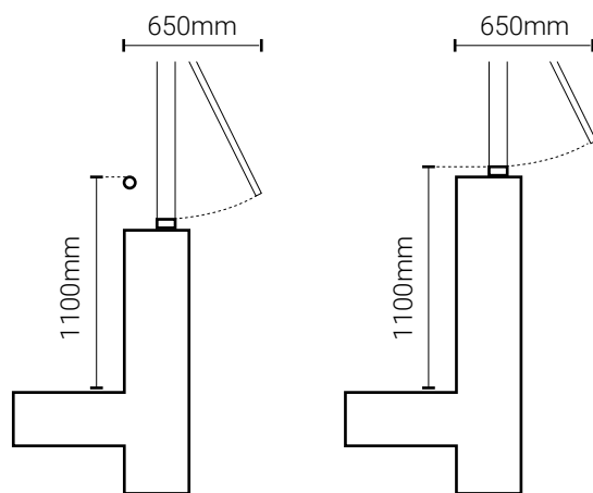
Figure 9. Illustrations of guarding meeting the standards of Table 3.1 (courtesy of AHMM).
