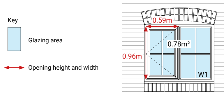
Figure 34. Glazing measurements taken for the kitchen window in the example home.
